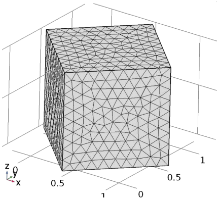
(c) No electric field applied, cube faces (110), ( \bar{1}10 ) and (001)
